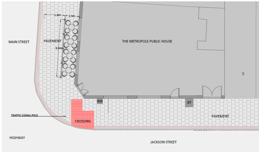
SITE PLAN @ 1 : 1250 (North Up)
